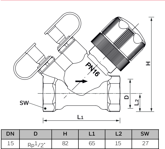
V5032...BLF Kombi-2-plus (DN15)
